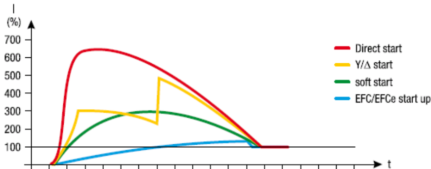
Start-up current with and without EFC/EFCE
